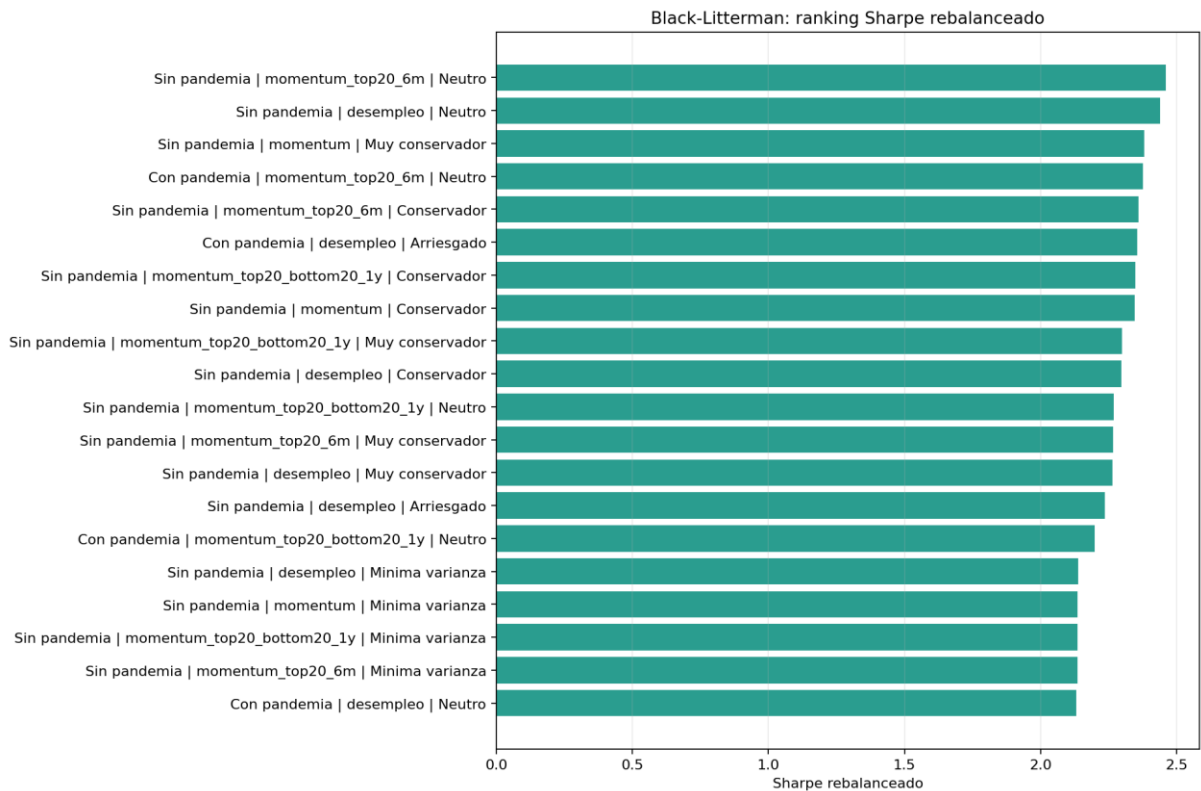
Figura 8. Ranking de Sharpe Black-Litterman.
